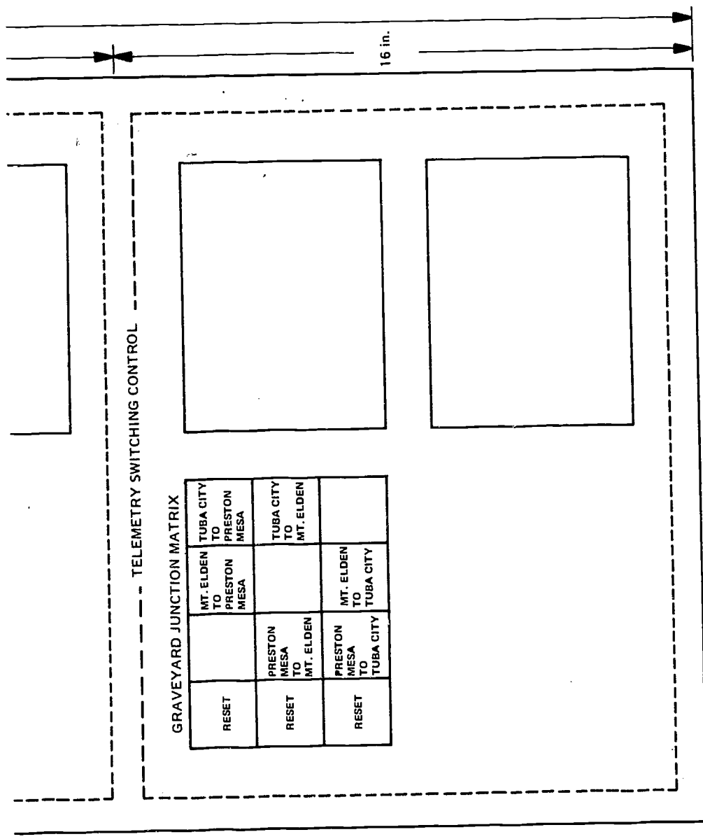
Figure D.6. Switching and Control Panel Layout at Tuba City.
