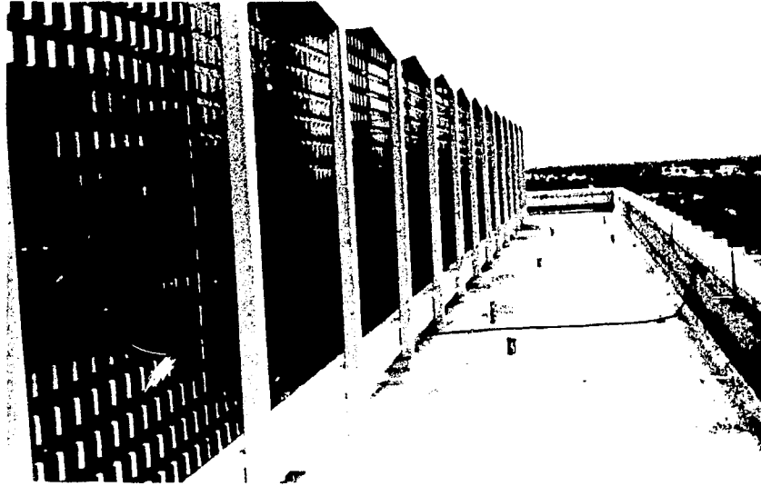
Figure C.1. Phoenix Indian Medical Center Roof Showing Lightning Rod Ground System and Grillwork Surrounding the Penthouse.
