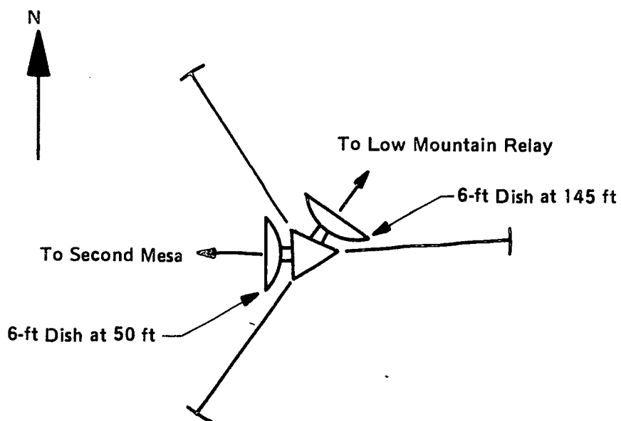
Figure D.7. New Antenna and Tower Arrangement at Keams Canyon Relay.
