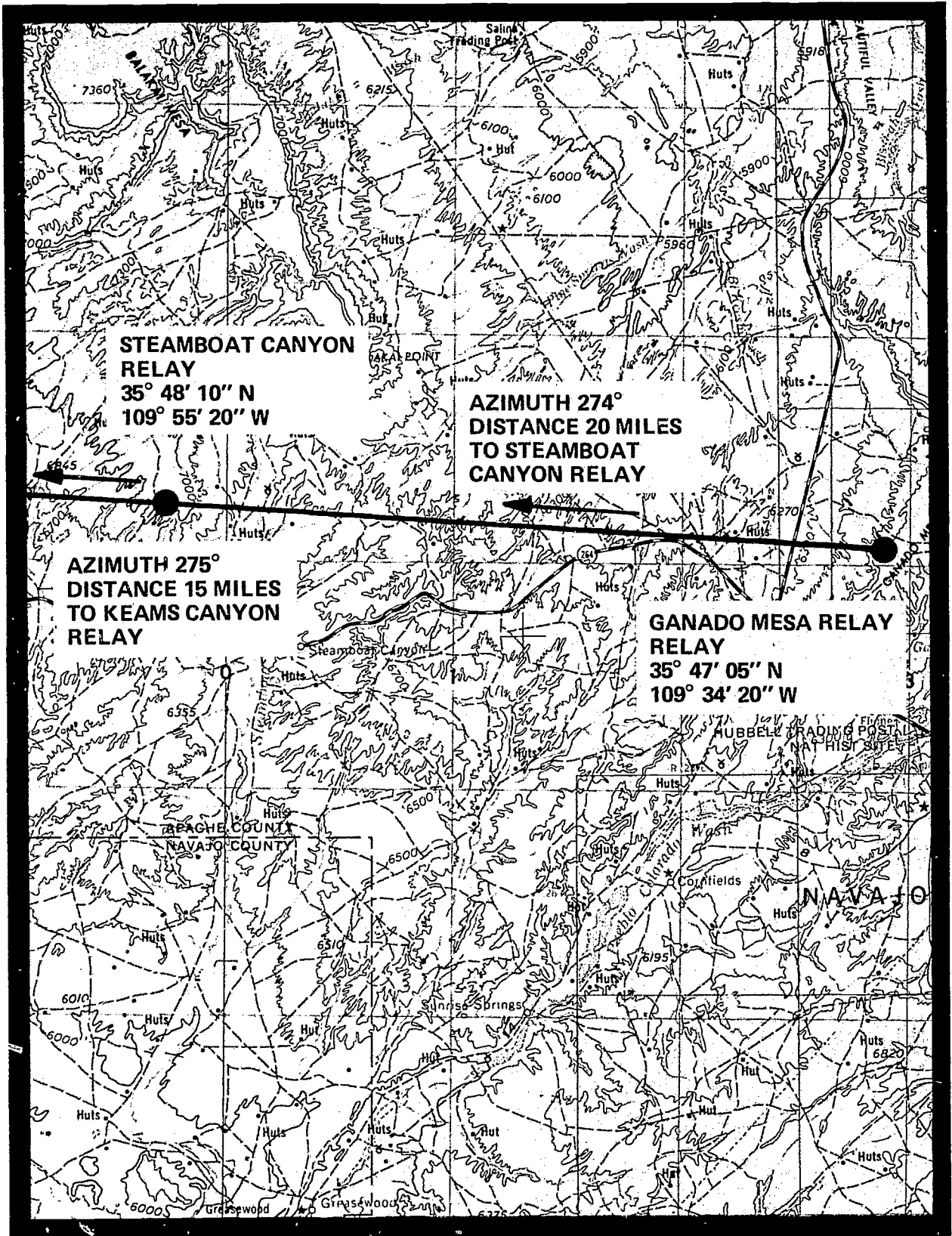
Figure B.2. Site Map Showing Steamboat Canyon Relay and Ganado Mesa Relay.
