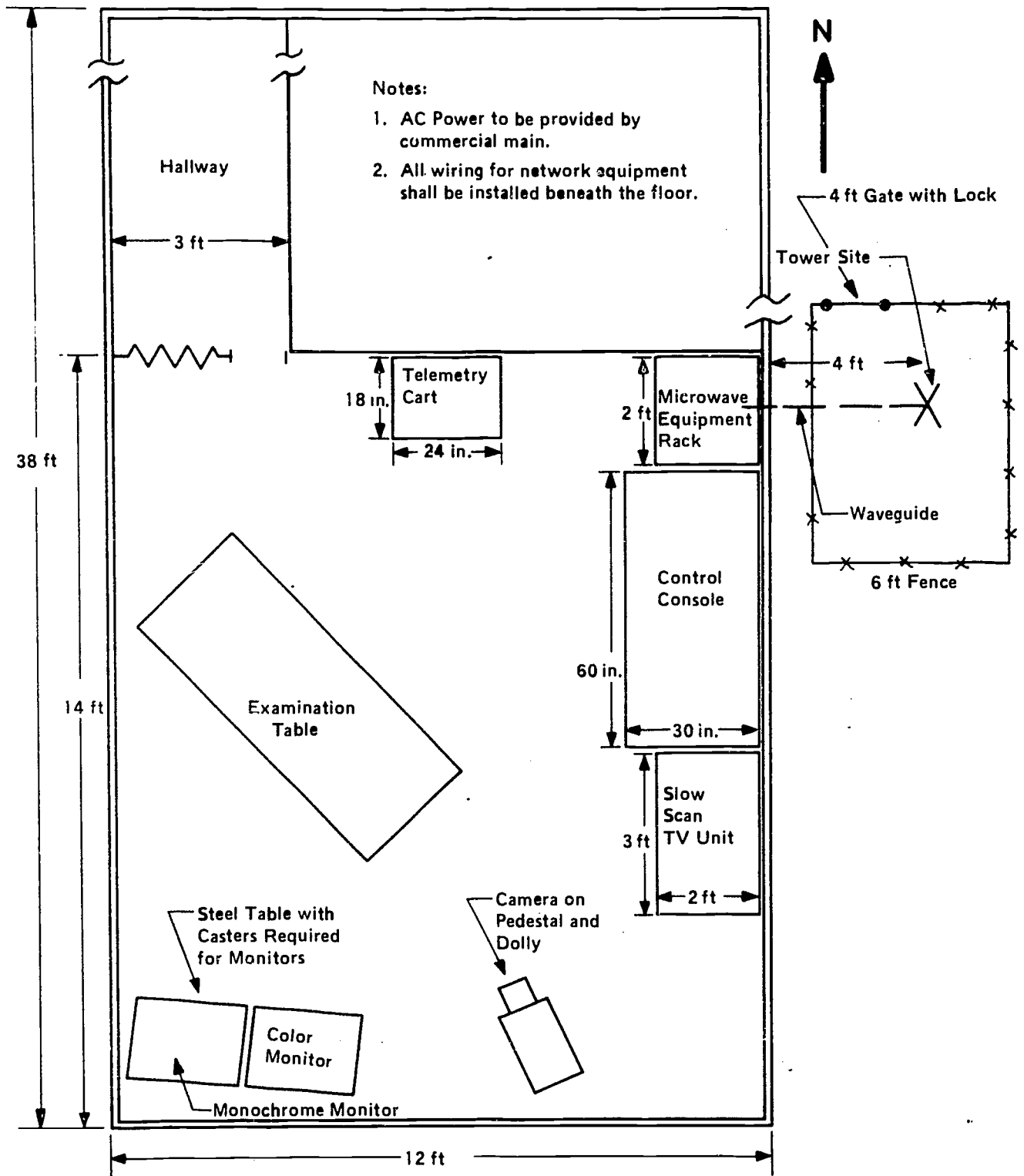
Figure D.2. Proposed Facilities at Shonto.
