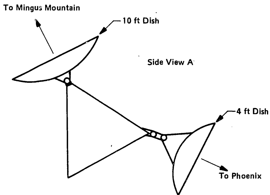
Figure D.14. New Tower and Antenna Arrangement at Shaw Butte.
